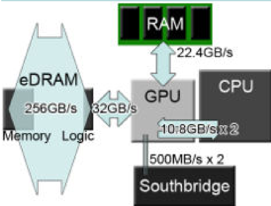
Xbox 360 Bandwidth Diagram
