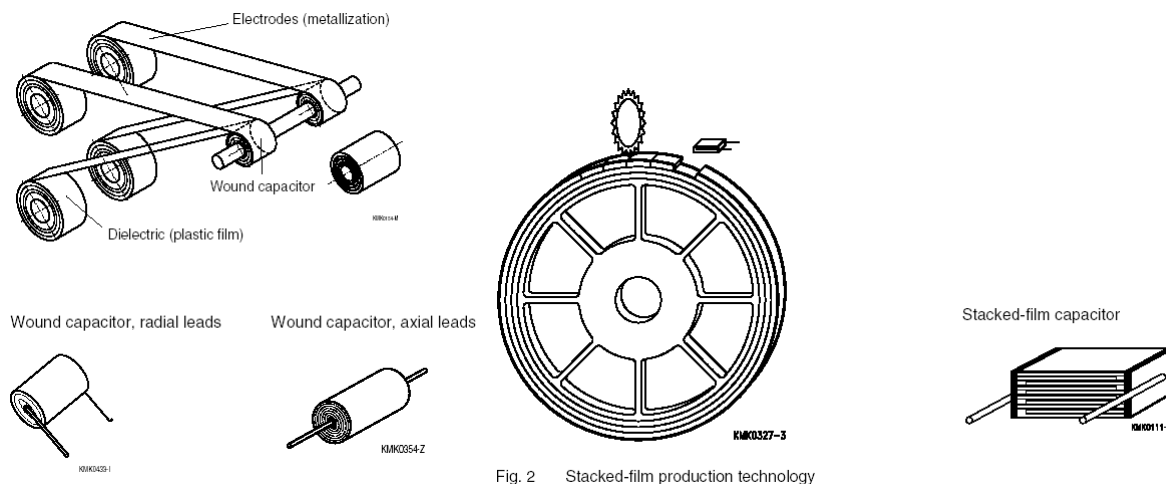
Fig. 2 Stacked-film production technology
