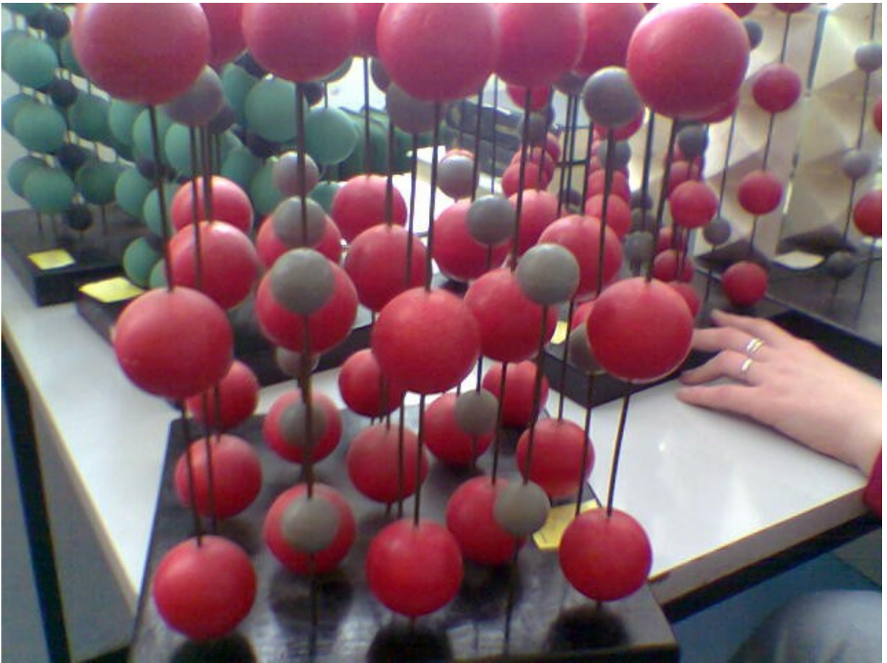
PbO
