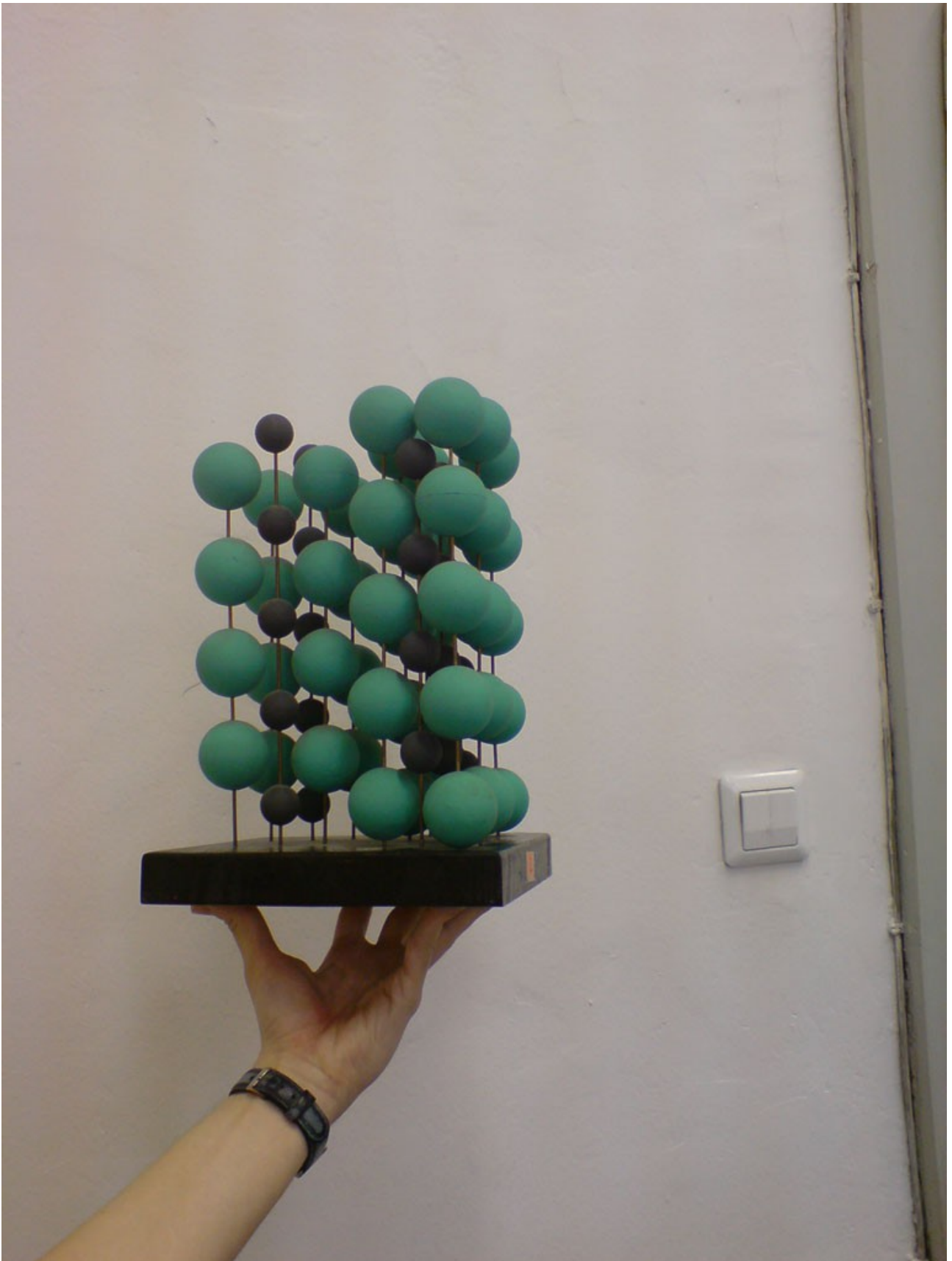
\text{PdCl}_2
