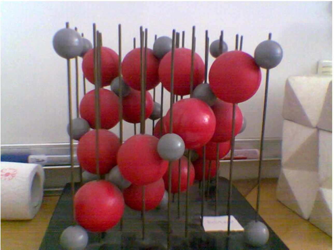
\text{SiO}_2 - kristobalit
