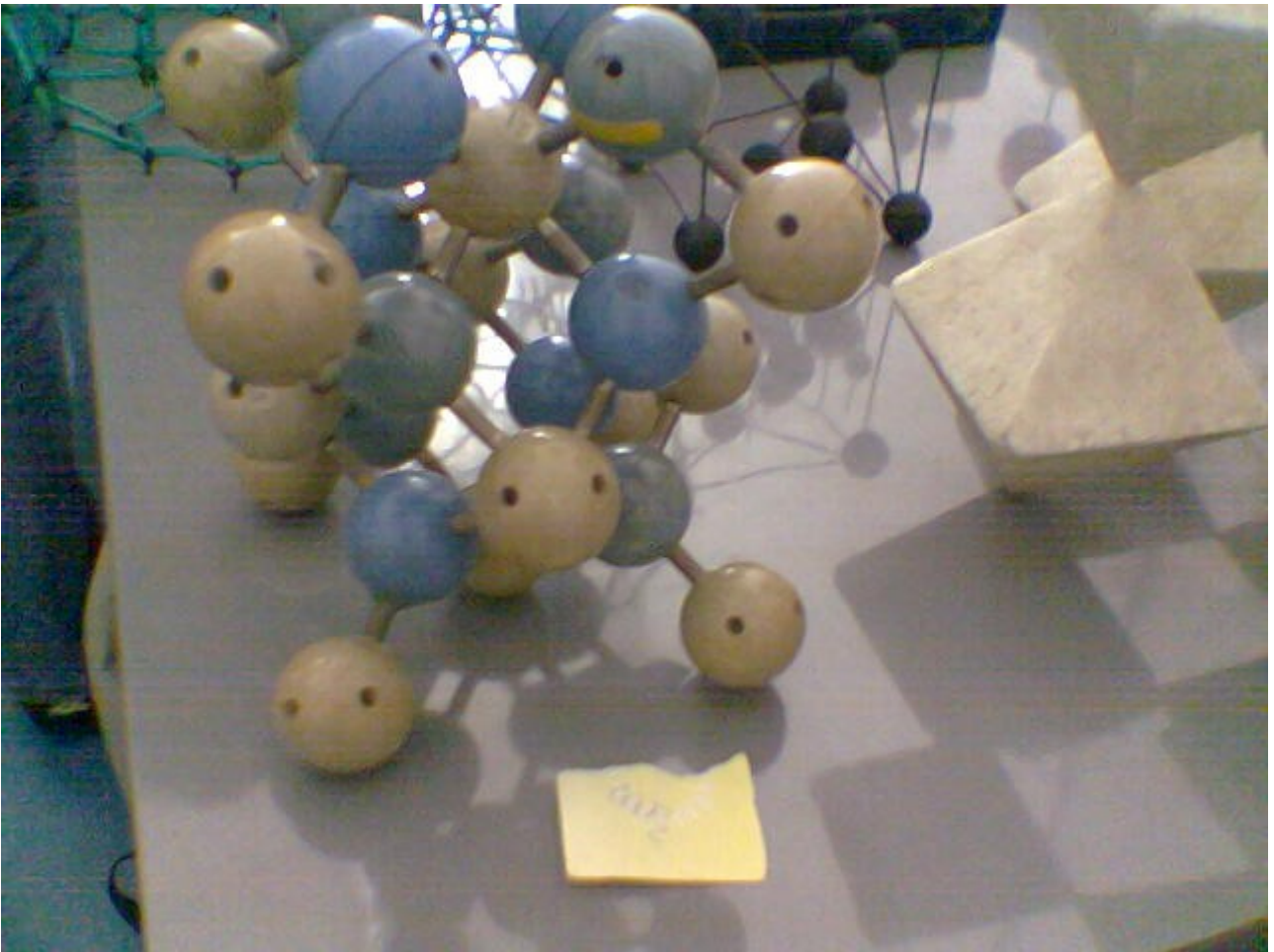
CaF 2
