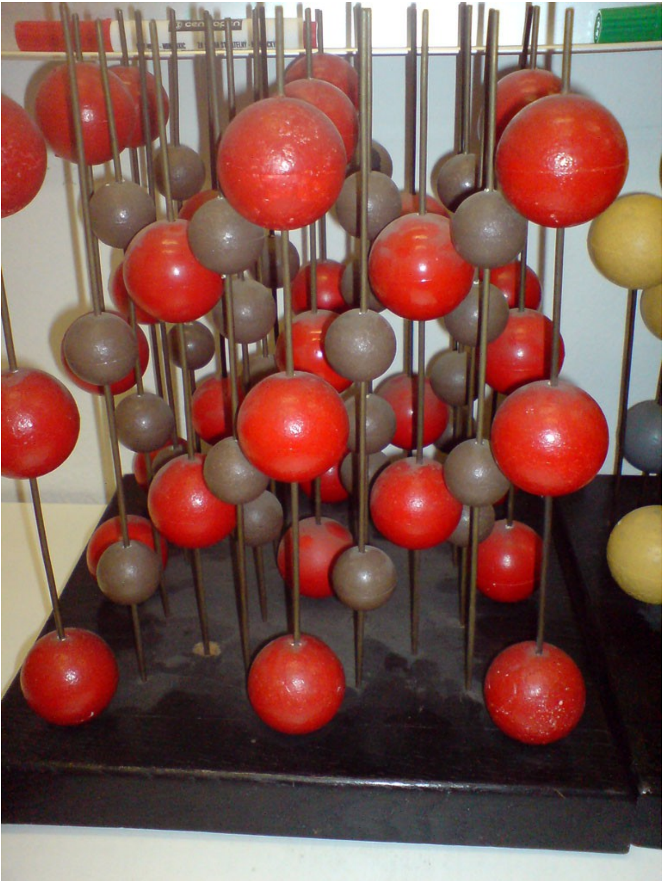
\text{Cu}_2\text{O}
