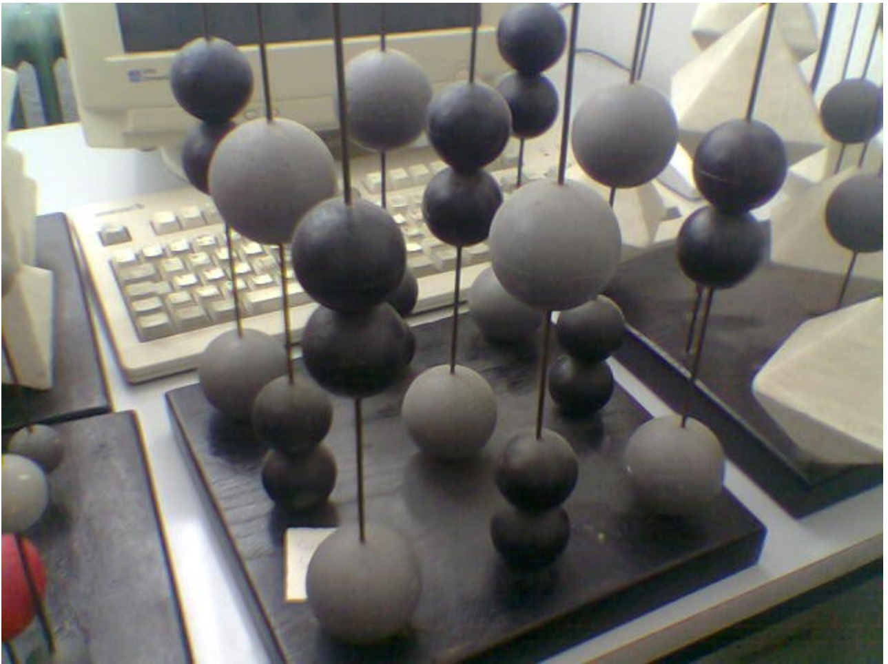
\text{CaC}_2
