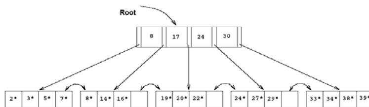
Figure 9.10 Example of a B+ Tree, Order d=2
