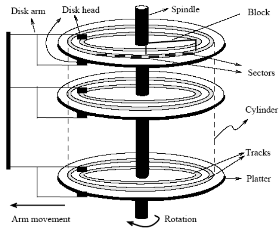
Figure 7.2 Structure of a Disk
