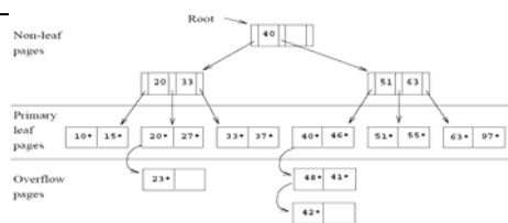
Figure 9.6 ISAM Tree after Inserts
