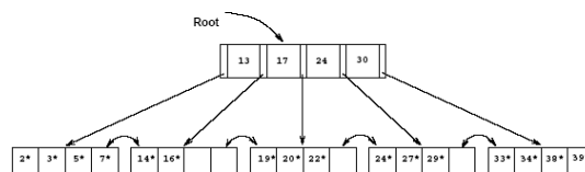
Figure 9.10 Example of a B+ Tree, Order d=2
