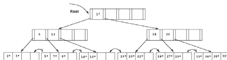
Figure 9.10 Example of a B+ Tree, Order d=2
