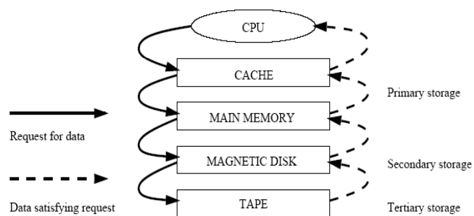
Figure 7.1 The Memory Hierarchy
