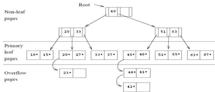
Figure 9.6 ISAM Tree after Inserts
