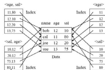
Figure 8.6 Composite Key Indexes
