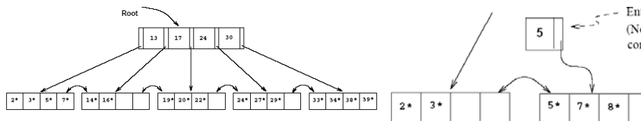
Figure 9.10 Example of a B+ Tree, Order d=2
