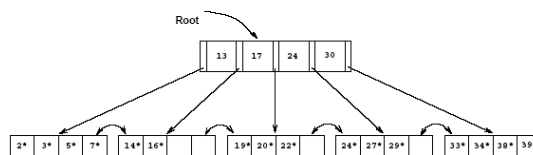
Figure 9.10 Example of a B+ Tree, Order d=2
