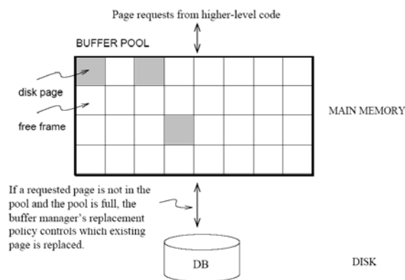
Figure 7.3 The Buffer Pool
